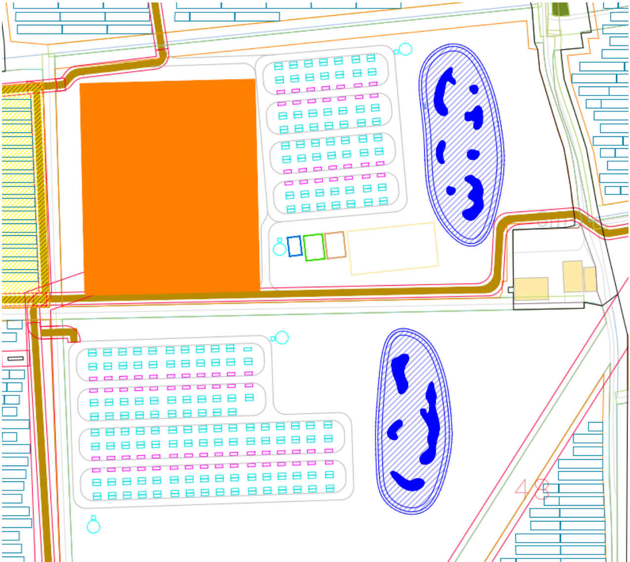
Figure 2.2: Illustrative Layout East BESS Site
