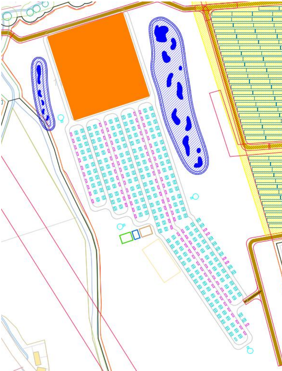
Figure 2.1: Illustrative Layout West BESS Site
